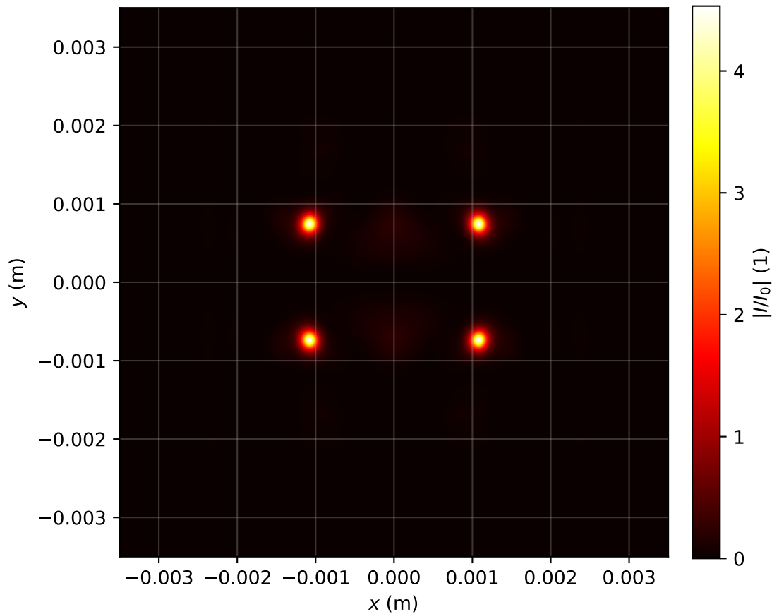
Intensity profile I(x, y, z = 2.548)/I_0 , P_{in}=7.0P_{cr} , artificial time
